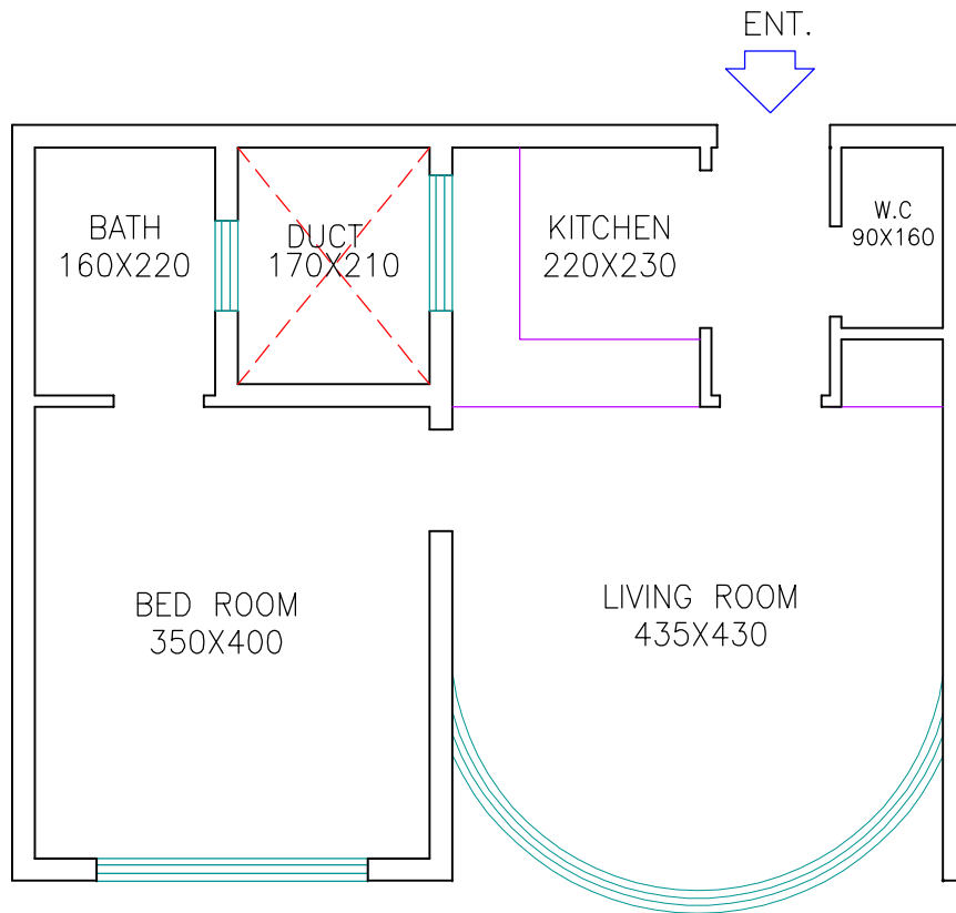
B2 PLAN ONE BED ROOM
